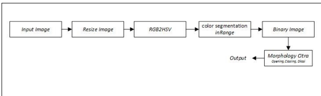
Figure 3. Pre-processing Stages
